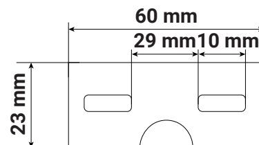
Fixing diagram
